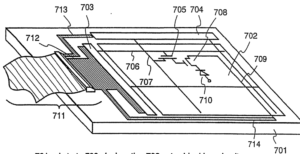
701:substrate 702:pixel portion 703:gate side driver circuit 704:source side driver circuit 705:switching TFT 706:gate wiring 707:source wiring 708:current control TFT 709:current supply line 710:EL element 711:FPC 712-714:connection wiring
